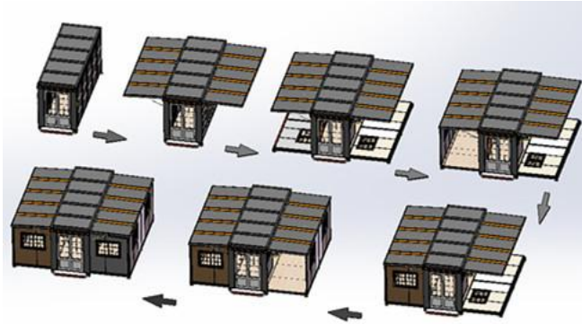
Installation process
