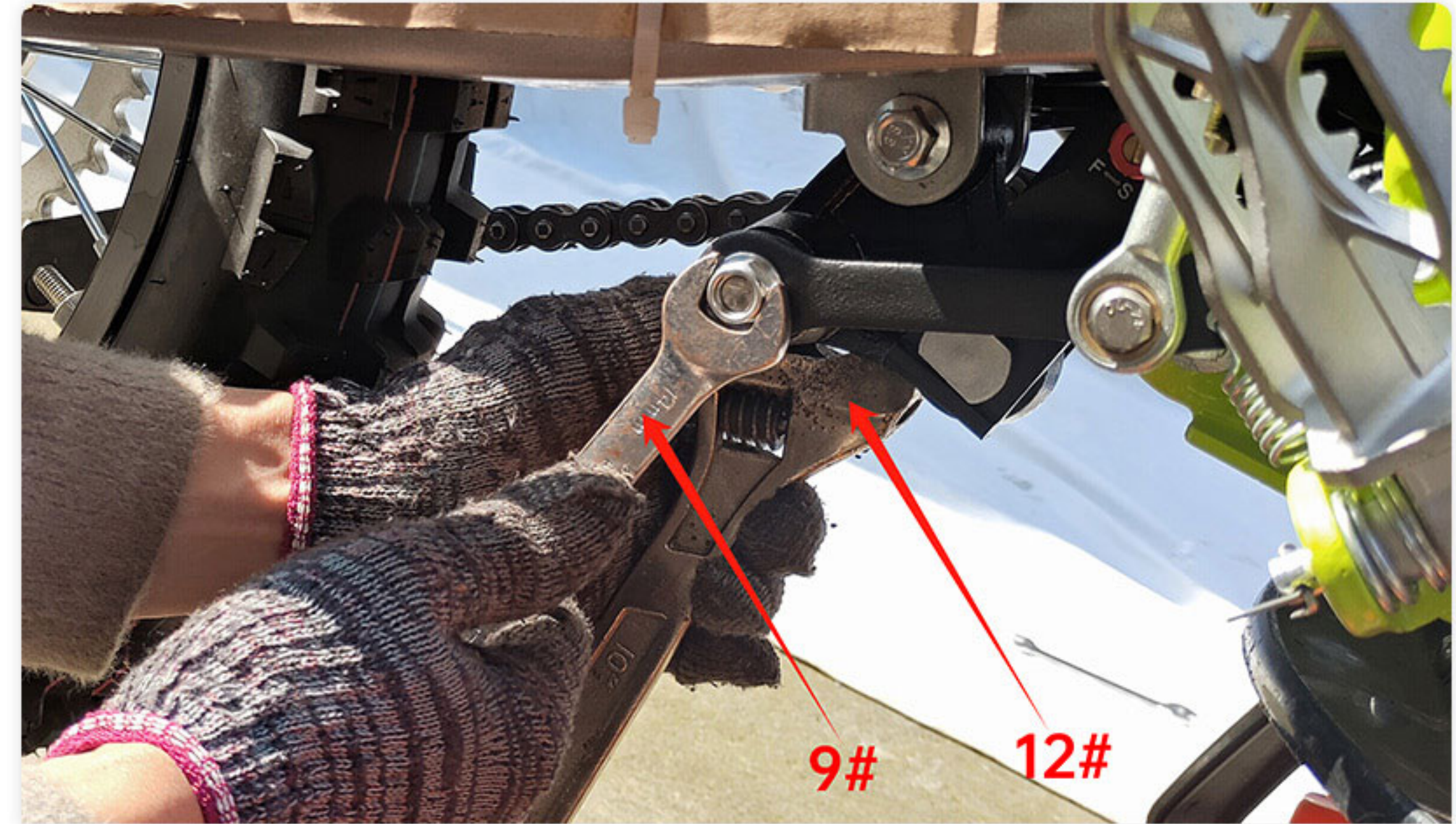
18. Using 9# 12# tool assemble Linkage Arm and Triangle Lever Linkage,lock the screws tightly
