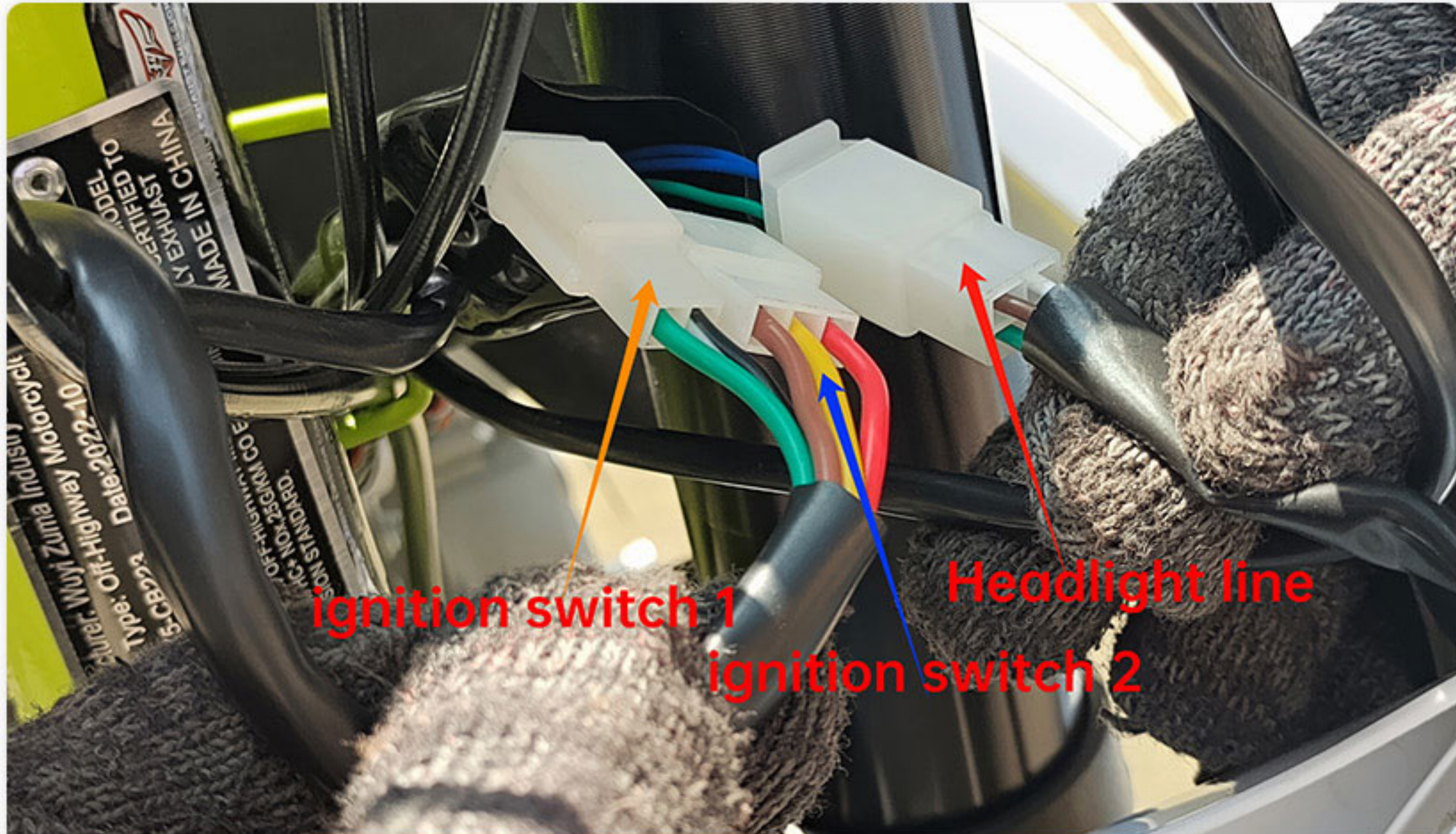
25. plug the ignition switch and wire harness as graph
