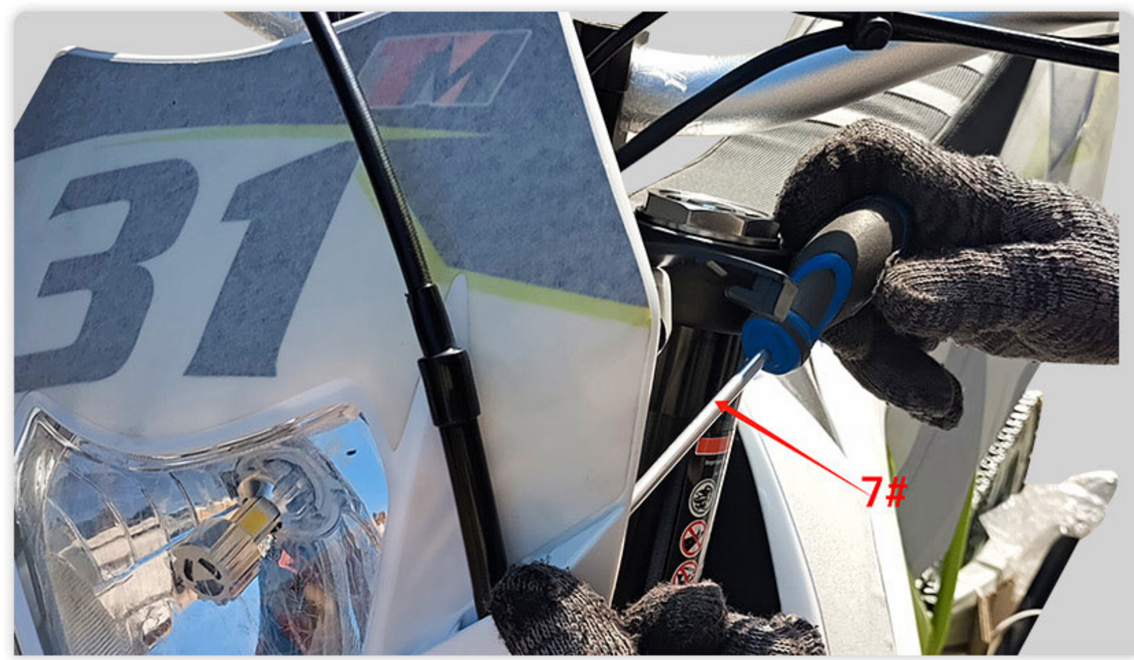
24. Assemble the front brake hose and bracket on headlight Using 7# tool
